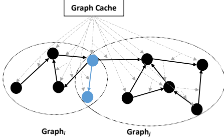
Figure 2: Illustration of cache containing responses to two queries with partial overlap.
