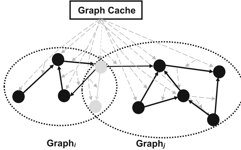
Fig. 2. Cache containing responses to two queries with partial overlap.
