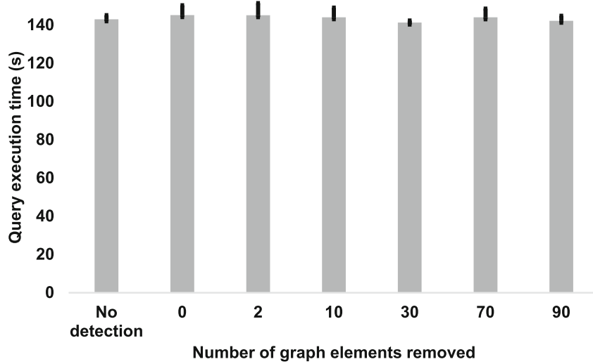
Fig. 8. Query execution time with discrepancy detection for a lineage query.
