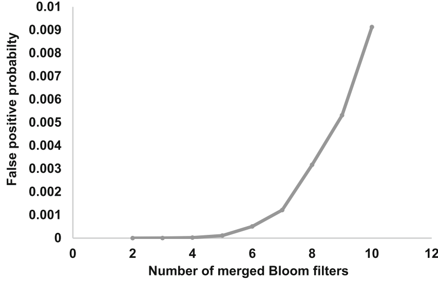
Fig. 7. False positive rate using merged Bloom filters.
