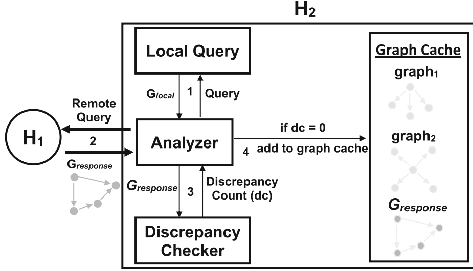
Fig. 4. Querying and discrepancy detection workflow.
